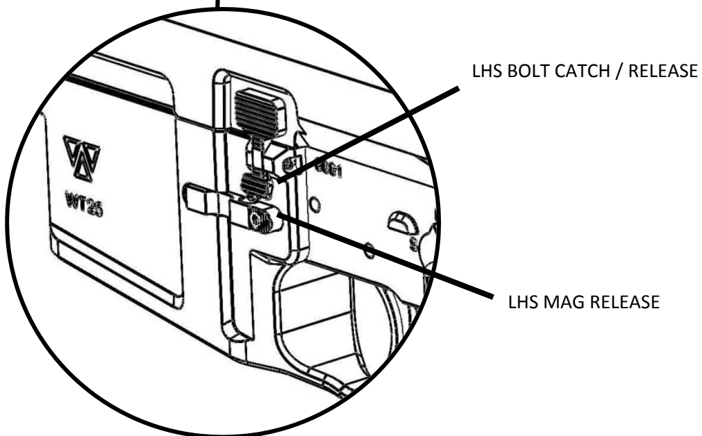
Left hand side mag release and bolt catch / release
