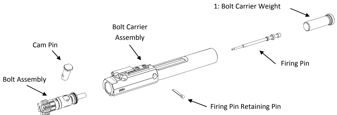
Figure 10: Field Stripped Bolt Carrier Group
