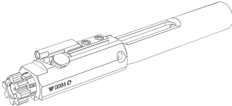
Bolt closed – cam pin in the rearward position
