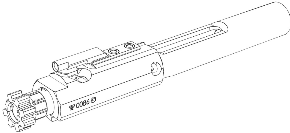
Bolt open – cam pin in the forward position, ready to be inserted into the rifle
